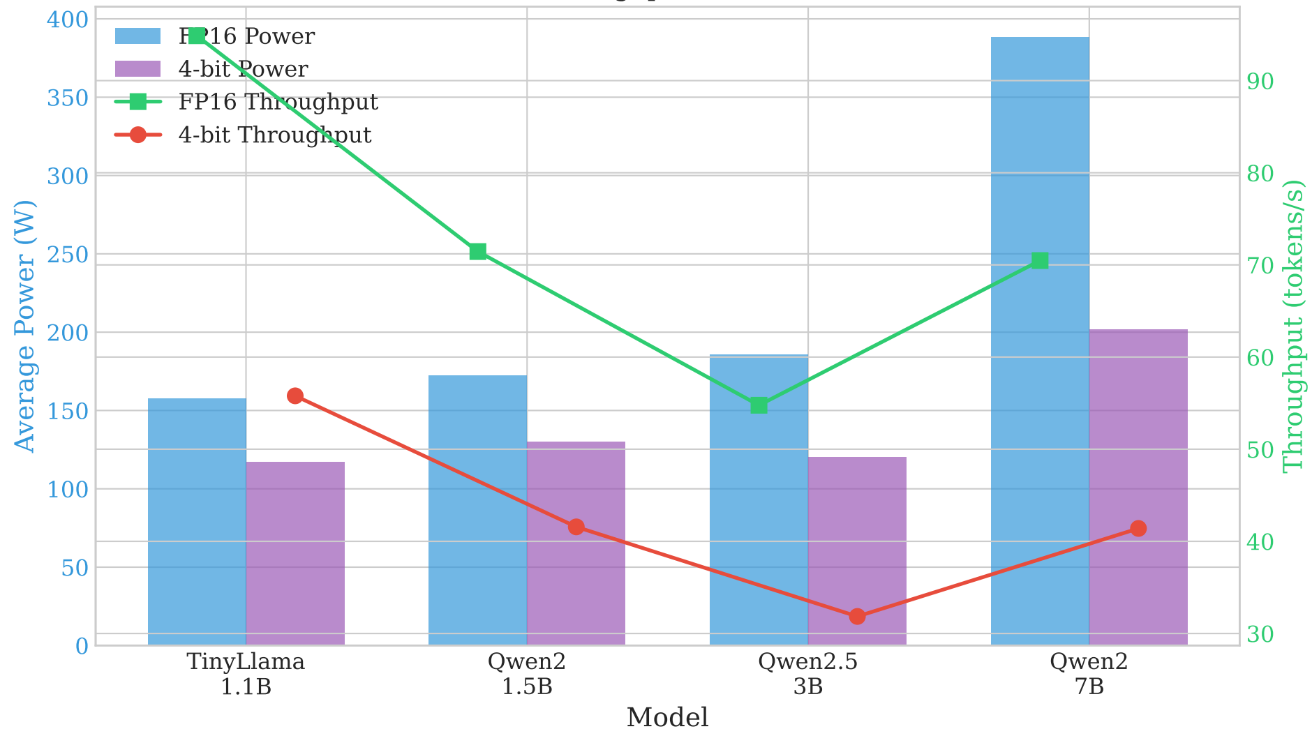
Power and Throughput: FP16 vs 4-bit NF4
