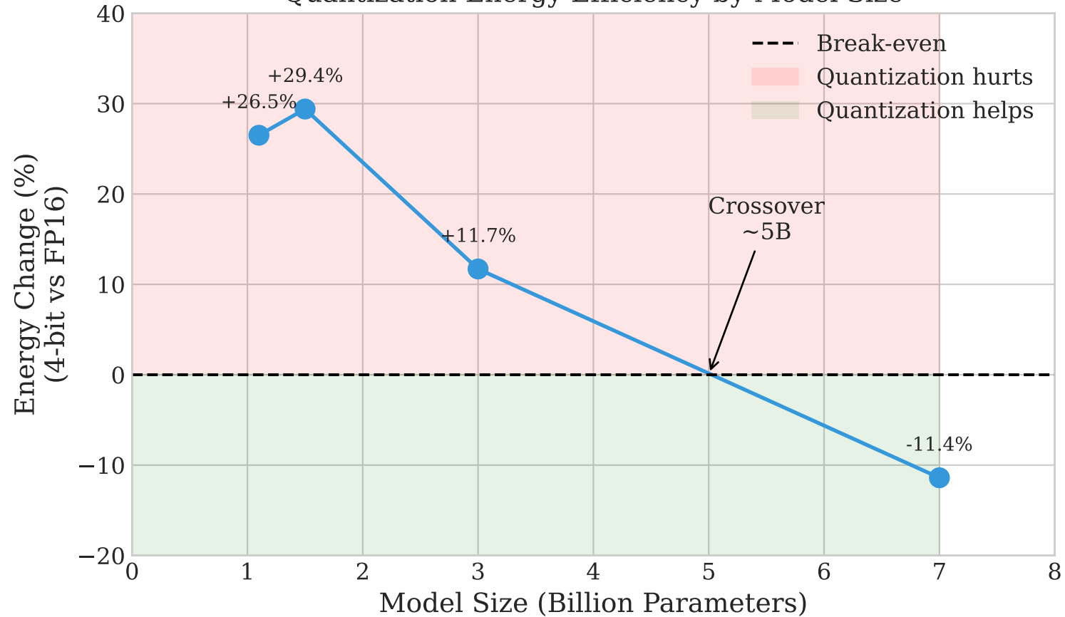
Quantization Energy Efficiency by Model Size
