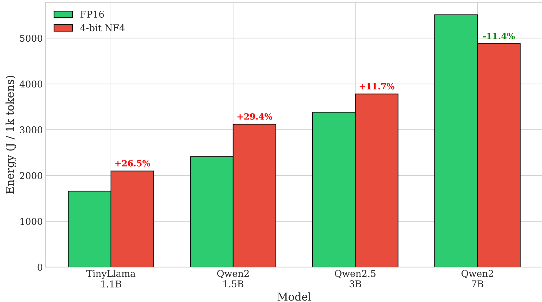
Energy Consumption: FP16 vs 4-bit NF4 on RTX 5090
